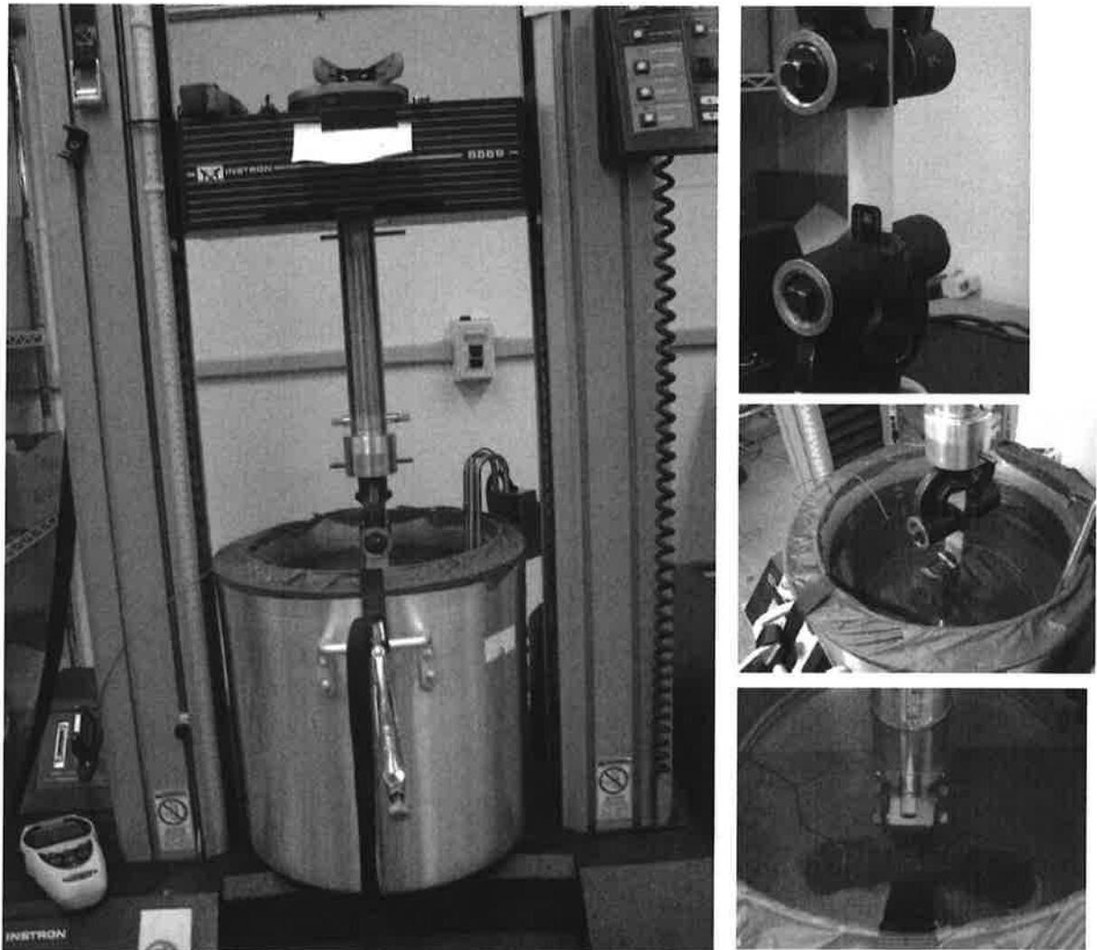
Figure 8. Left - Instron with heated water bath and clamped nylon strap. Right top - Air shear test. Right middle - Heated shear with added weights immersed in water to accommodate higher shear forces and unattached part of label bent to accommodate clamp. Right bottom - Heated peel test with visible orange thermocouple to monitor water temperature, floating roller peel fixture with white polypropylene test plate, and bottom fixed fixture epoxied to aluminum pot containing heated water.
